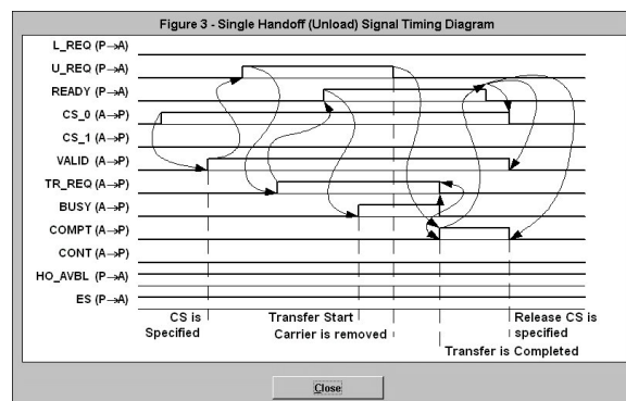
Single Handoff (Unload) Signal Timing Diagram
