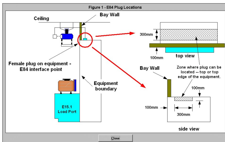
E84 Plug Locations
