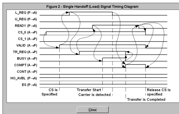
Single Handoff (Load) Signal Timing Diagram
