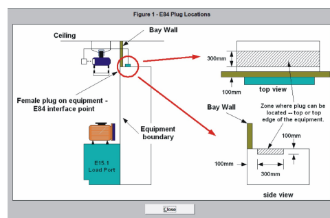
E84 Plug Locations
